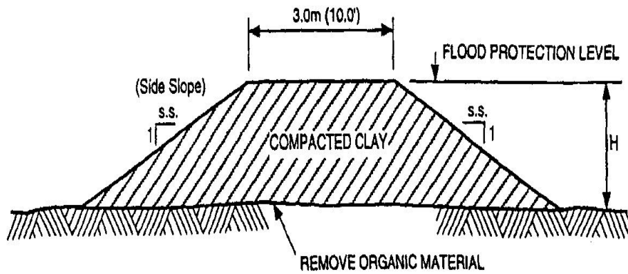
DIKE CROSS - SECTION (minimum elevations)
