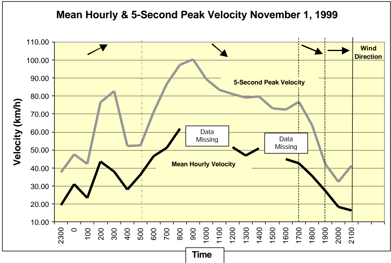
Figure 6.1: Wind velocities and directions, November 1, 1999, Delta Beach (Prepared by the Committee using weather data supplied by the Delta Marsh Field Station, University of Manitoba.)
