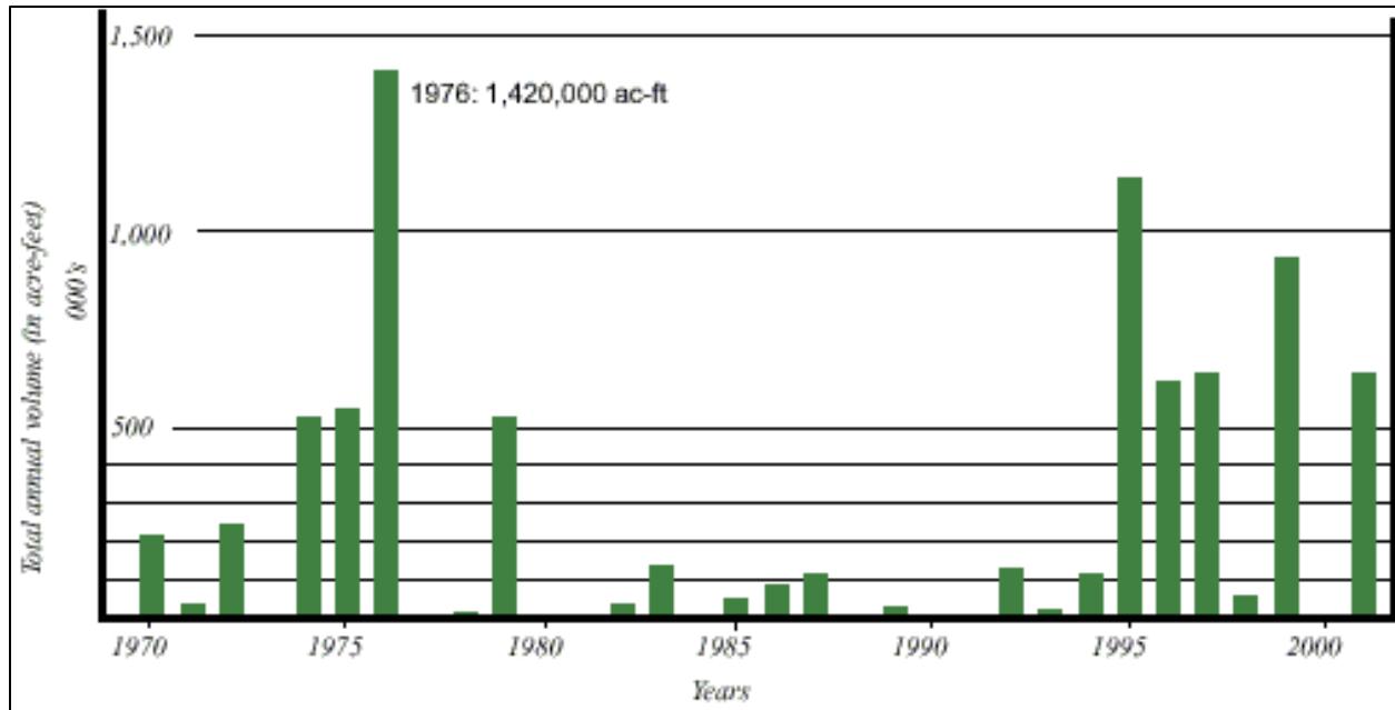
Figure 4.2: The Portage Diversion – Years of operation and flows.
