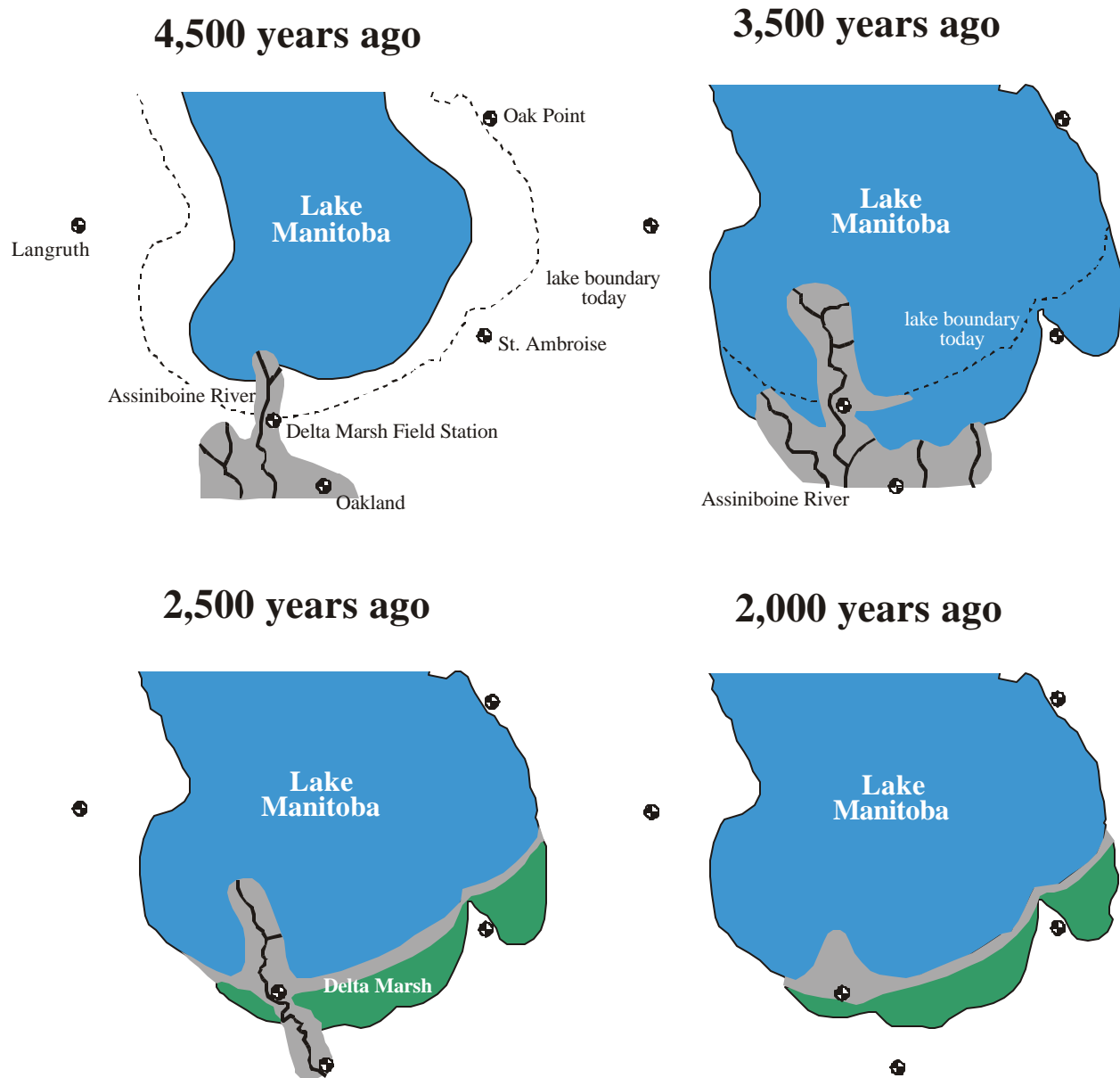
Figure 4.1. Reconstruction of changes in Lake Manitoba between 4,500 and 2,000 years ago, based on analysis of lake sediment from 51 sites in the south basin 15
