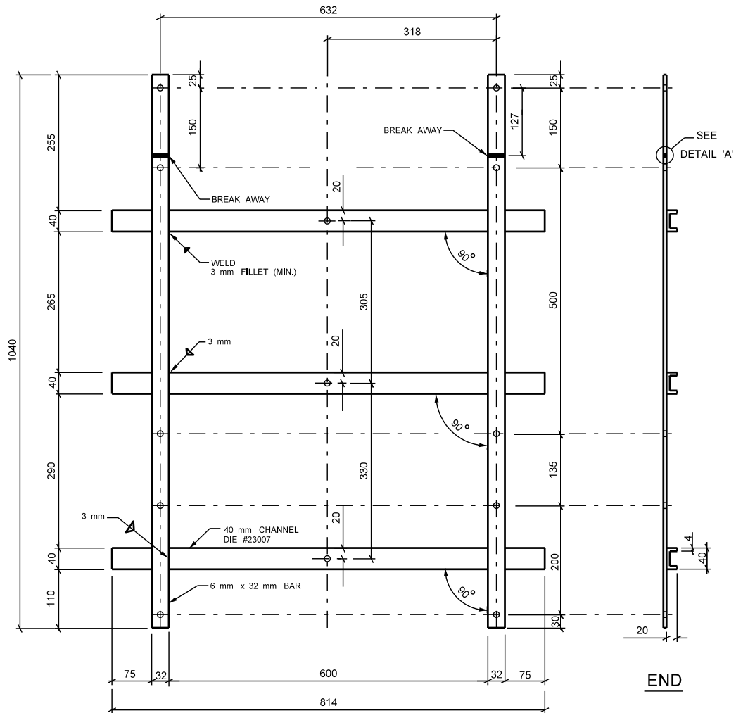
FRONT VIEW
