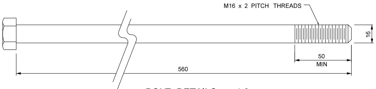
BOLT DETAILS 1:2
