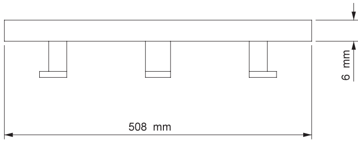
ELEVATION VIEW
