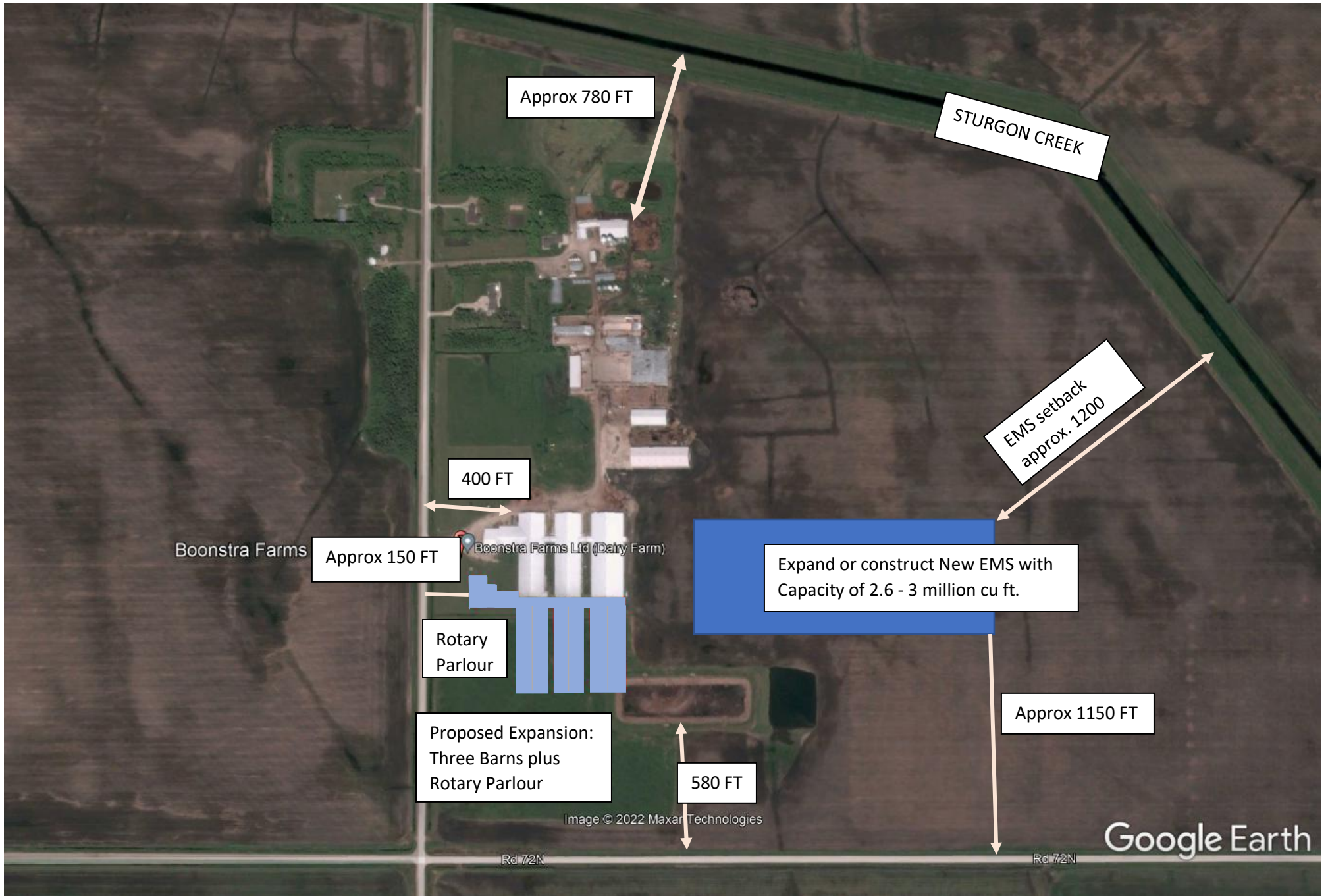
SITE PLAN – BOONSTRA DAIRY FARM LTD.
