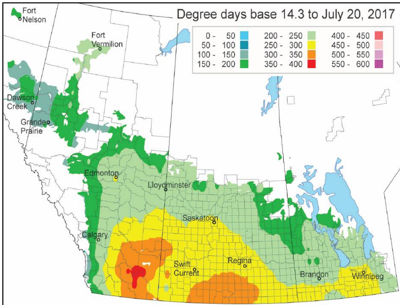
Figure 4 - Degree day accumulations, as of Week 29, across the Prairie Provinces (Map produced by Agriculture and Agri-Food Canada's Prairie Pest Monitoring Network).
