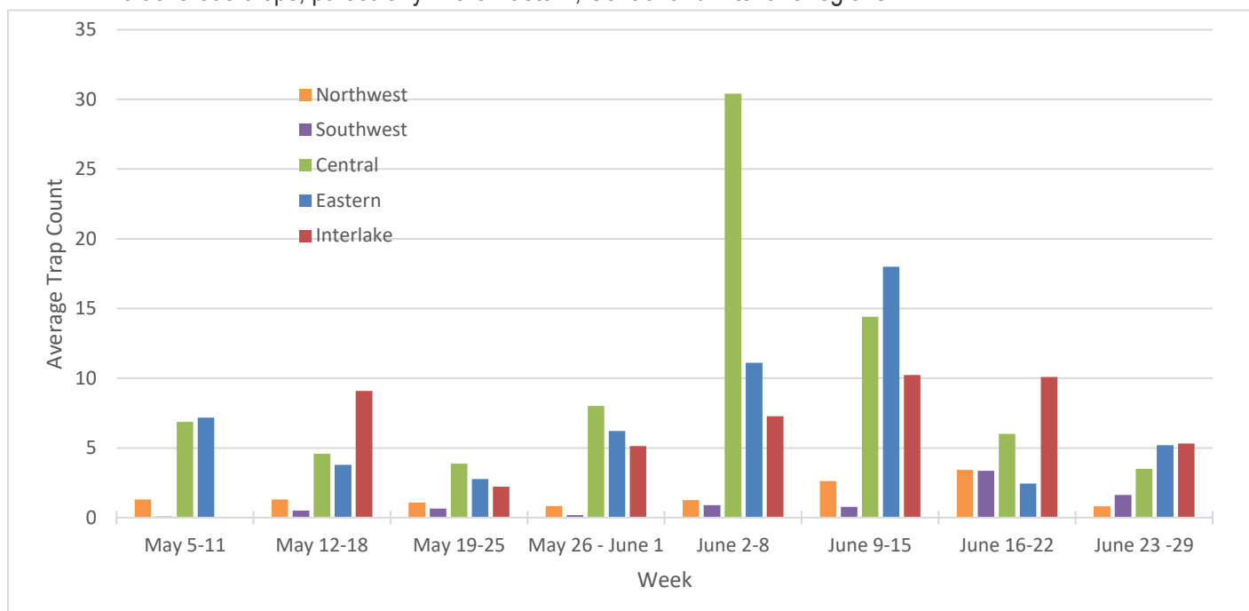
Figure 3. Average weekly trap counts for diamondback moth per agricultural region in Manitoba.
